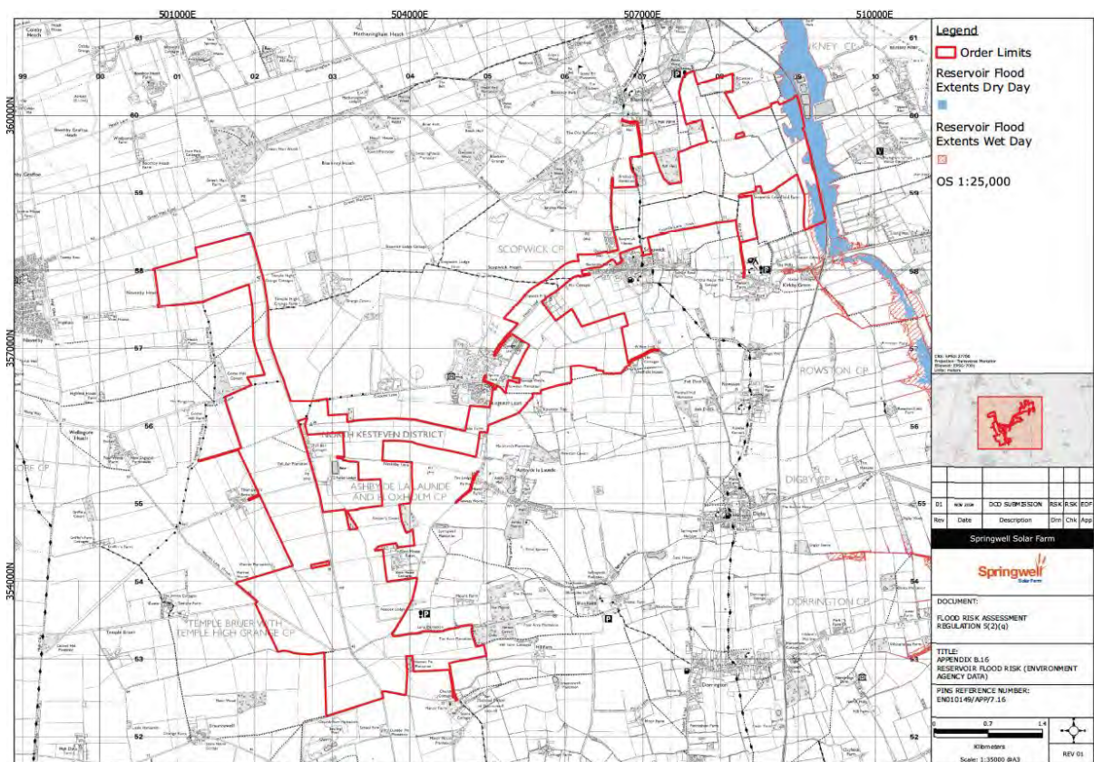
Plate 3.1764: Environment Agency reservoir flood extents (model layer from Defra) (full map in Appendix B.163)
