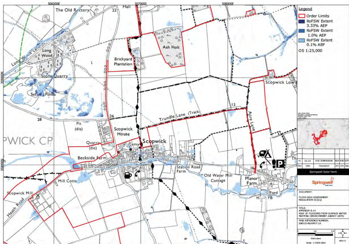
Plate 3.130: Surface water flood risk extents (5) (full map in Appendix B.144)
