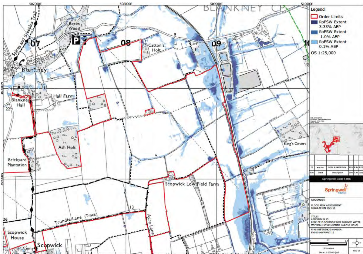
Plate 3.1443: Surface water flood risk extents (6) (full map in Appendix B.152)
