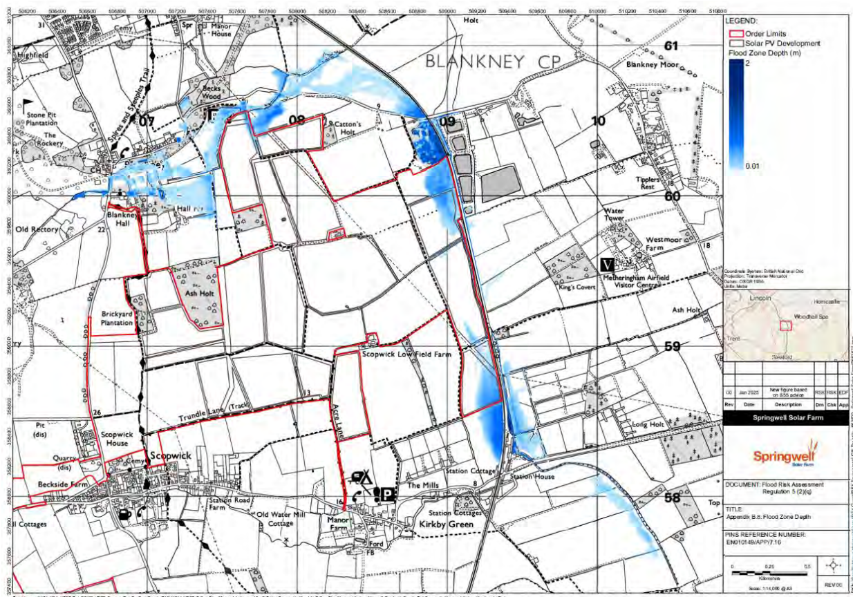
Plate 3.8: 3.8: Flood Depth Modelling (full map in Appendix B.8)
